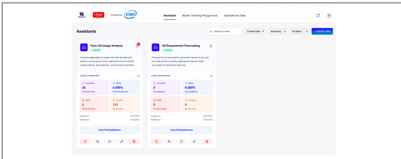
Figure 1. Assistant screens.
